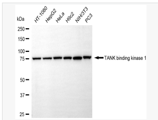
Western blotting analysis using TANK binding kinase 1 antibody (R020205). Total cell lysates (30 \mu g) from various cell lines were loaded and separated by SDS-PAGE. The blot was incubated with TANK binding kinase 1 antibody (R020205, 1:5,000) and HRP-conjugated goat anti-rabbit secondary antibody (1:20,000) respectively. Image was developed using ECL Substrate Kit.
