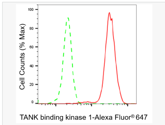
Flow cytometric analysis of TANK binding kinase 1 expression in HepG2 cells using TANK binding kinase 1 antibody (R020205, 1:2,000). Green, isotype control; red, TANK binding kinase 1.
