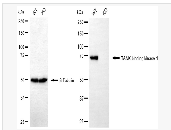
Western blotting analysis using TANK binding kinase 1 antibody (R020205). TANK binding kinase 1 expression in wild-type (WT) and TANK binding kinase 1 (TBK1) knockout (KO) 4T1 cells with 20 \mu g of total cell lysates. \beta -Tubulin serves as a loading control. The blot was incubated with TANK binding kinase 1 antibody (R020205, 1:5,000) and HRP-conjugated goat anti-rabbit secondary antibody (1:20,000) respectively. Image was developed using ECL Substrate Kit.
